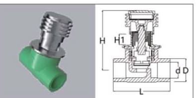
Plastic Valve with Brass
