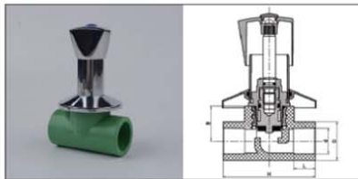
Concealed Valve
