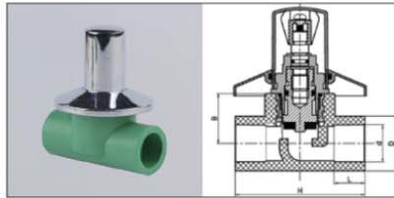
Concealed Valve(Short)
